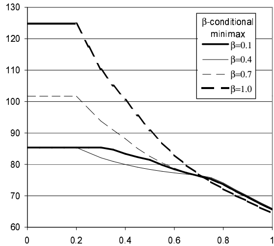
Fig. 2. Curves of the worst conditional means.
