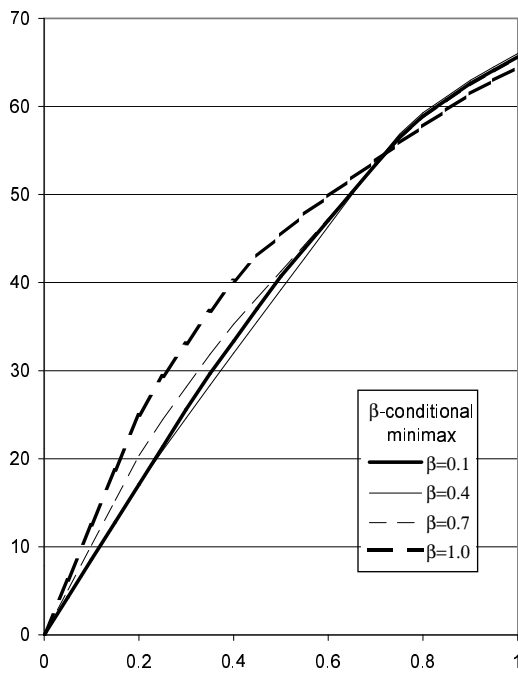
Fig. 3. Absolute Lorenz curves for the sample problem.
