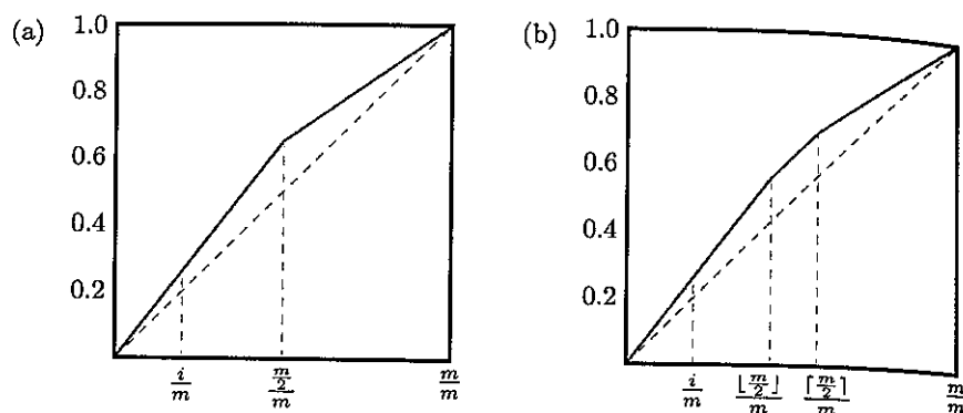
Fig. 1. Areas under Lorenz curve for minimal maximum deviation: even (a) vs. odd (b) number of weights
