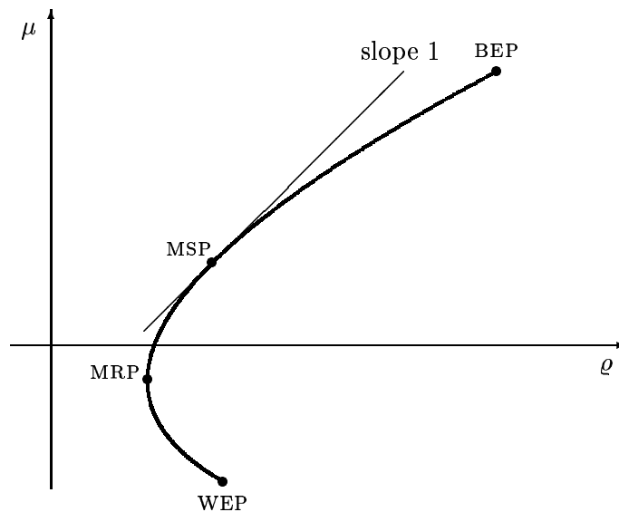
Figure 1: The mean-risk analysis
