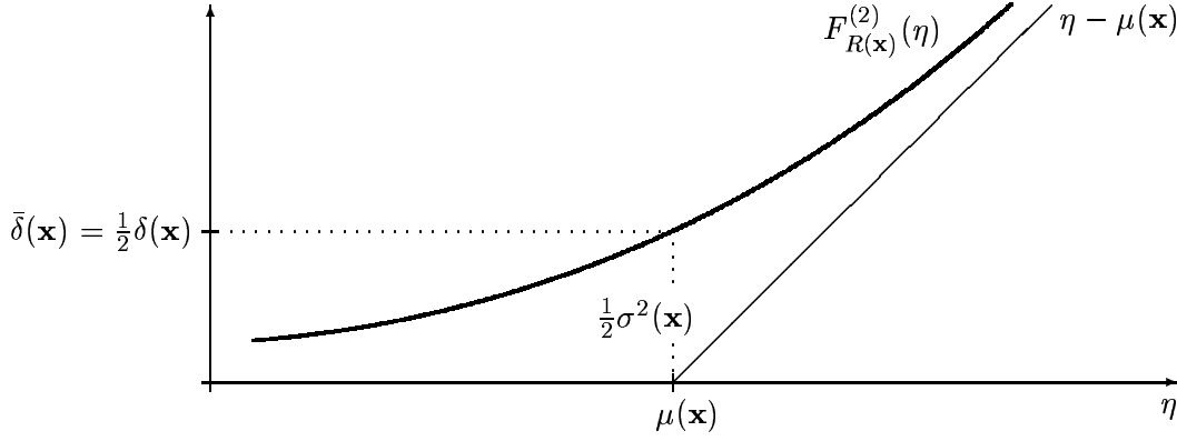
Figure 2: The O–R diagram
