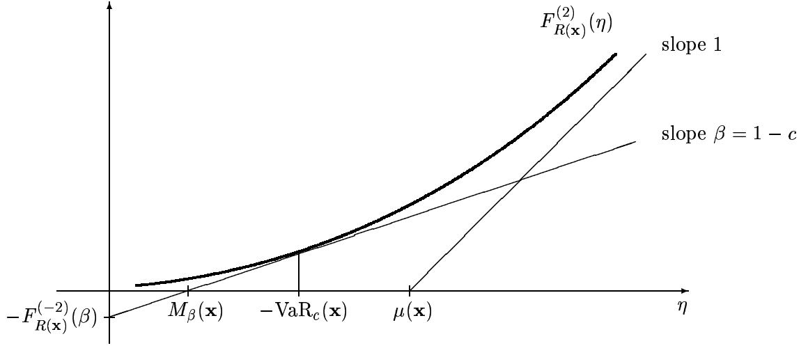
Figure 5: Quantile safety measures in the O-R diagram
