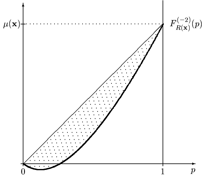
Figure 3: The absolute Lorenz curve and the dual dispersion space
