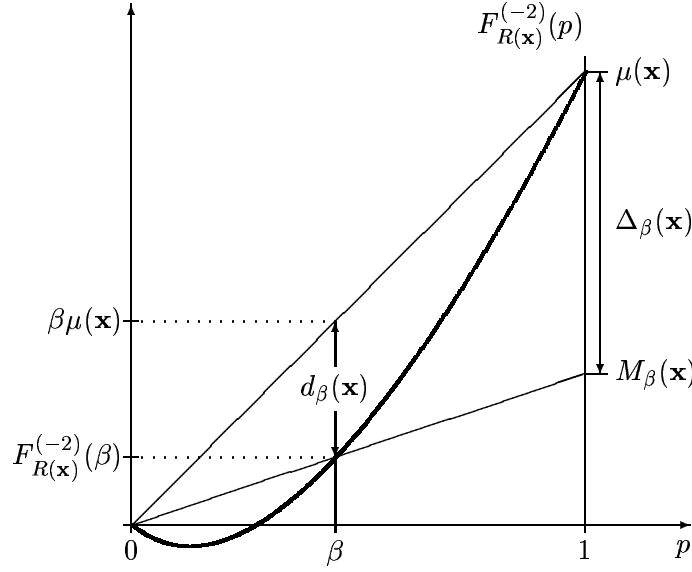
Figure 4: The absolute Lorenz curve and the conditional worst realizations
