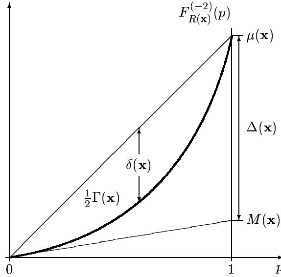
Figure 6: The absolute Lorenz curve and LP computable risk measures
