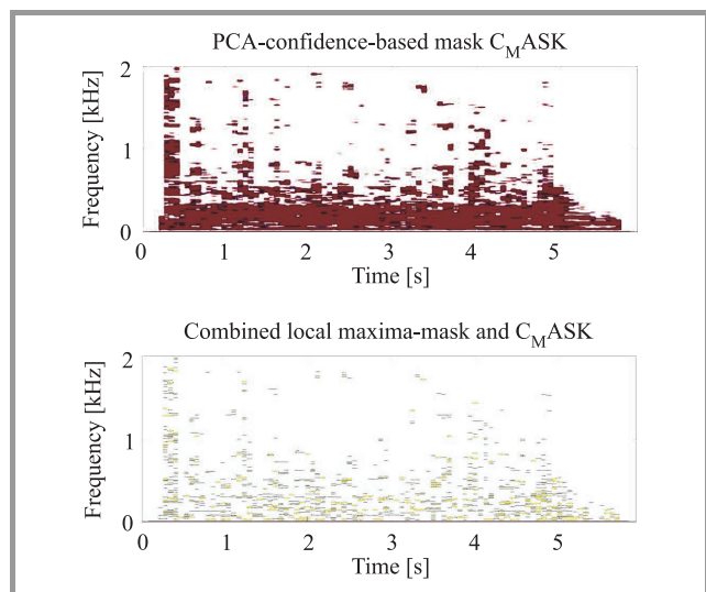
Fig. 5. Selection mask for spectrogram cells based on confidence value (top), compared with energy-based selection mask (bottom) (for real mixtures).
