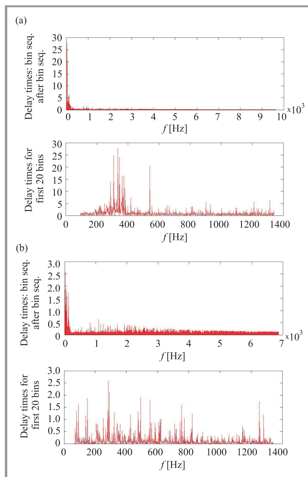
Fig. 2. Time delays as a function of frequency: (a) in real mixtures and (b) simulated mixtures.
